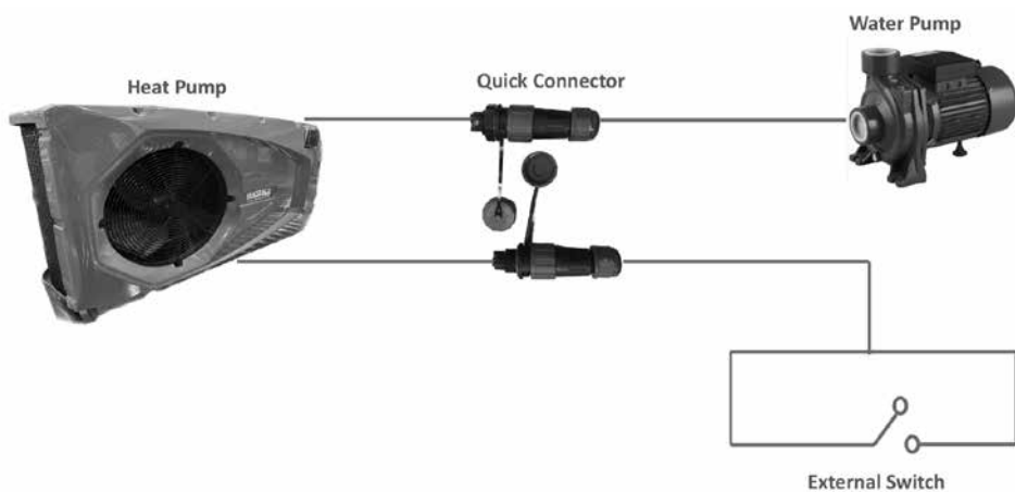
External Switch
